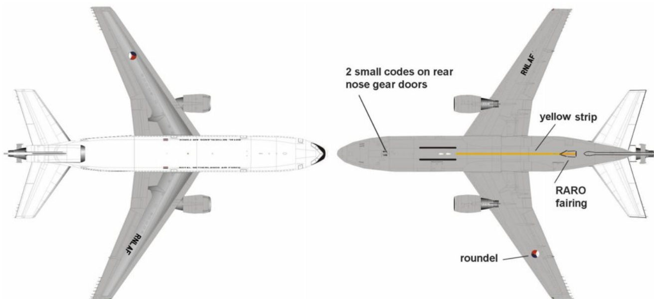
STANDARD UPPER AND LOWER VIEWS (note stabilizer white colour)
